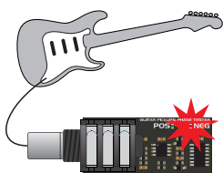
A guitar with reversed phase pickups
